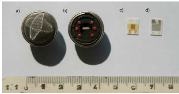
Fig. 1. Taguchi gas sensors produced by Figaro company: (a) purchased sensor, (b) with uncovered gas sensitive layer and contacts, (c) a prototype of monosized nanoparticle gas sensor and (d) its platinum heater.
